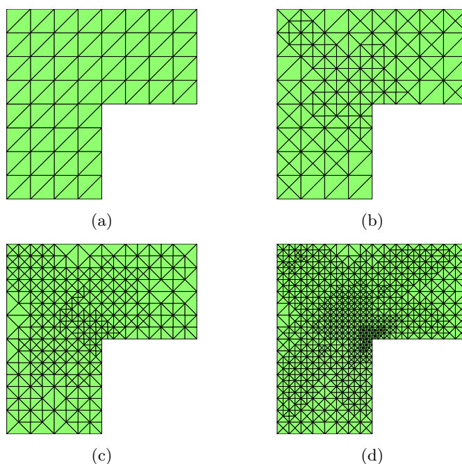
Fig. 4.2.: Coarse and fine grids for an L-shaped domain. Fig. 4.2a is the coarse grid. Fig. 4.2b, 4.2c and 4.2d
