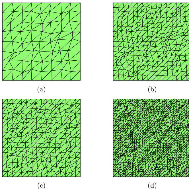
Fig. 4.1.: Unstructured 2D meshes
